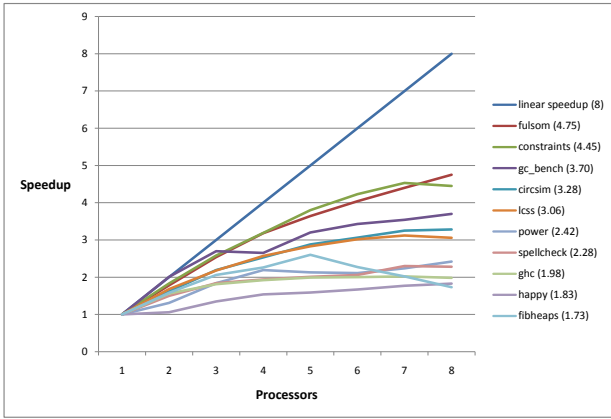
Figure 5. Speedup on various benchmarks
